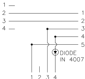
WIRING DIAGRAM
